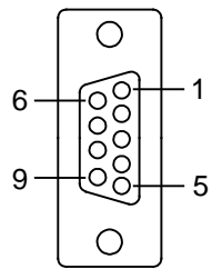
DB9 Male
