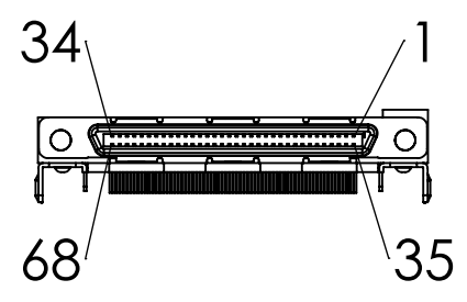
Connector Pinout (Both Female)
