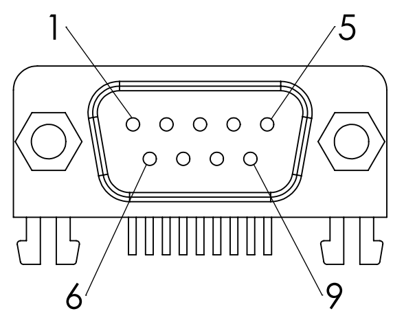
Connector Pinout (Male)
