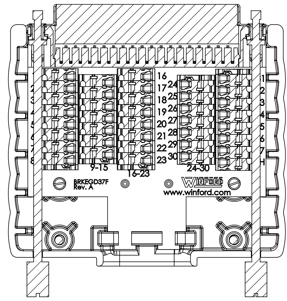
SECTION B-B
