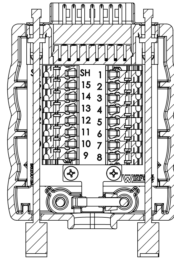
SECTION B-B
